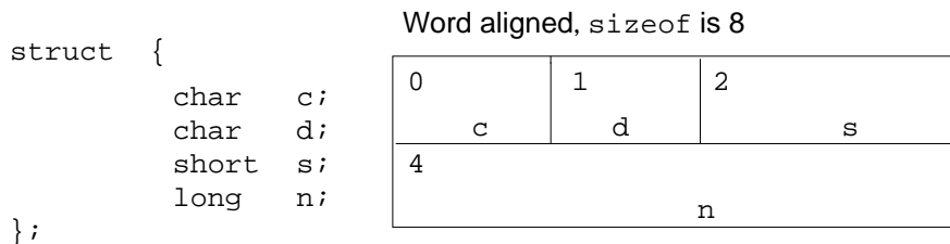
Figure 3-7 No Padding—Big-Endian
