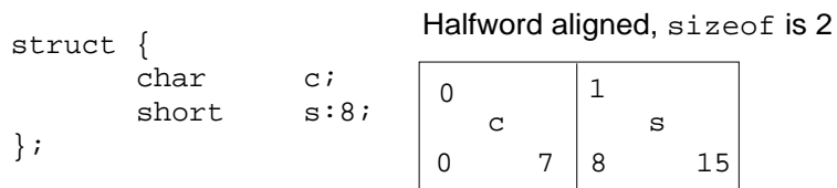
Figure 3-20 Storage Unit Sharing—Big-Endian
